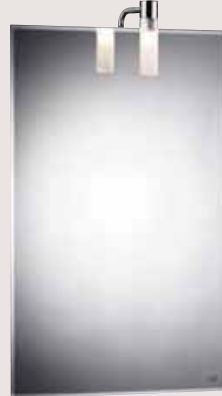
Standard bevelled mirror with fixings and optional 25w Halogen G9 lamp. Dimensions D1000mm x W600mm
